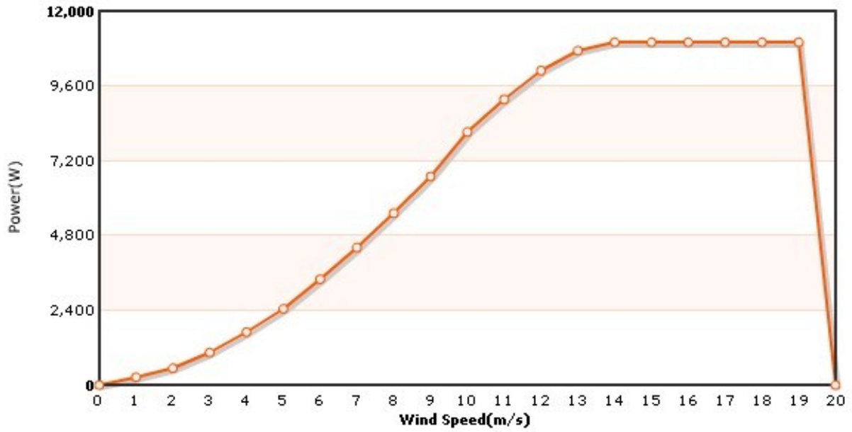
SKYWING 10K-G/SKYWING 10K-G3 CURVE
