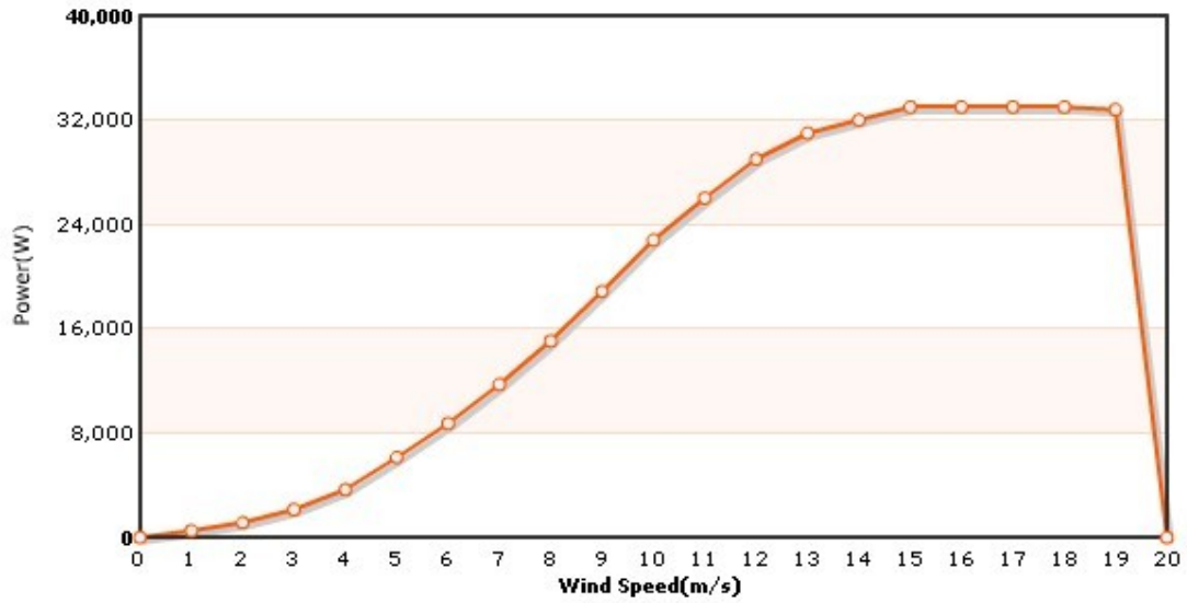
SKYWING 30K-G3 CURVE
